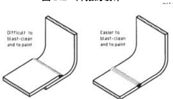
Figure D.2 — Design of welds
