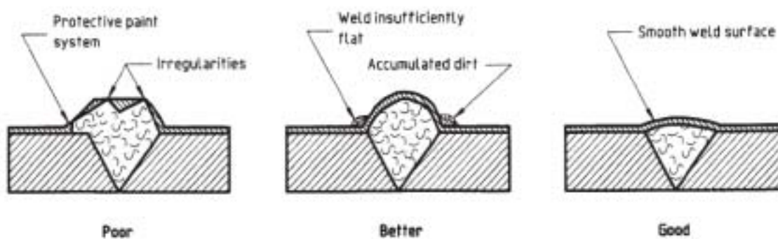
Figure D.6 — Avoidance of welding surface imperfections
